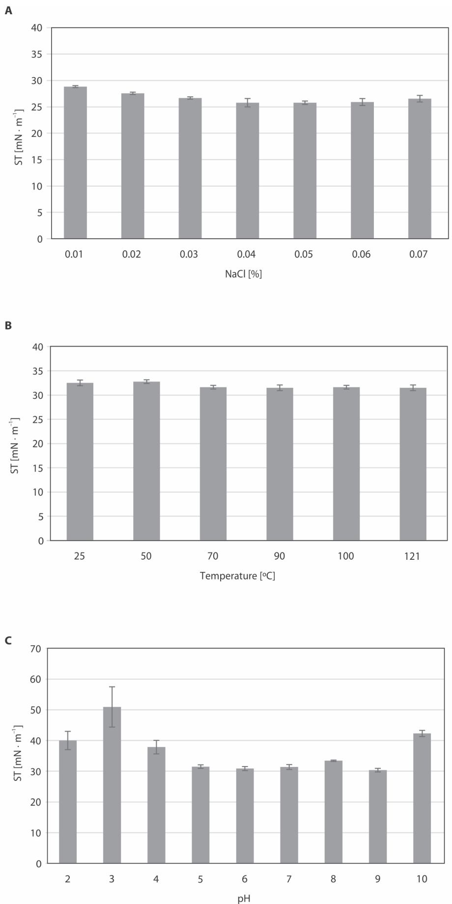
Fig. 2A-C. Stability of the surface-active properties of biosurfactants produced by Bacillus subtilis BS19 under different salinities – A, temperature – B and pH – C. The results represent the mean ± standard deviation. ST – surface tension
